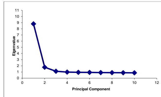
P-6. Mathematics Grade 10 Principal Components Scree Plot
