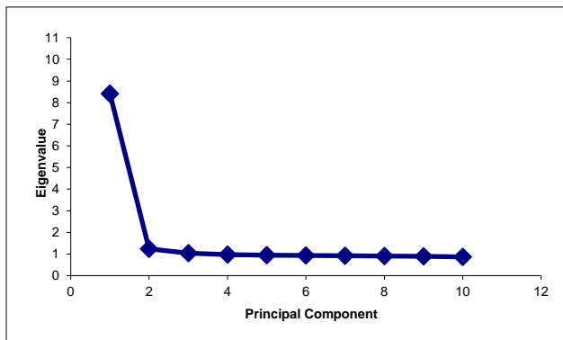
P-7. Science Grade 9 Principal Components Scree Plot
