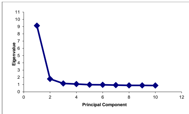
P-5. Mathematics Grade 9 Principal Components Scree Plot
