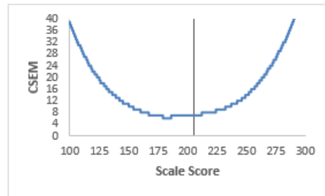
G-4. Reading Grade 10 Conditional Standard Error of Measurement
