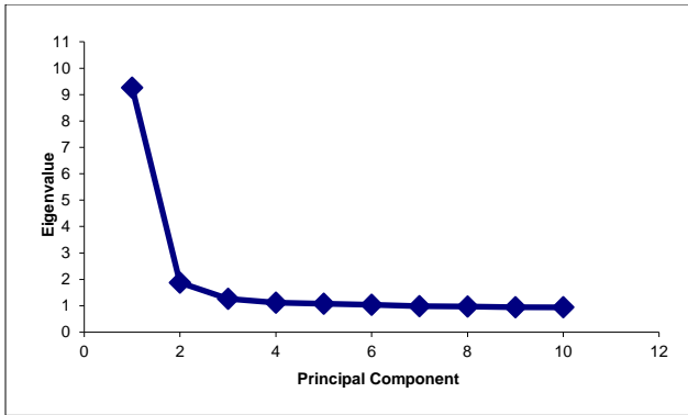
P-1. English Grade 9 Principal Components Scree Plot
