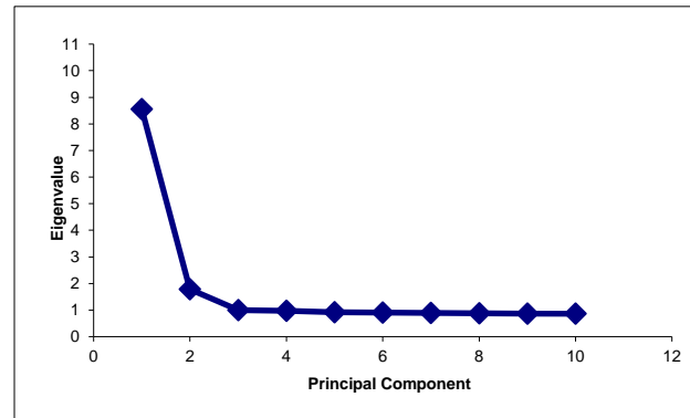
P-4. Reading Grade 10 Principal Components Scree Plot
