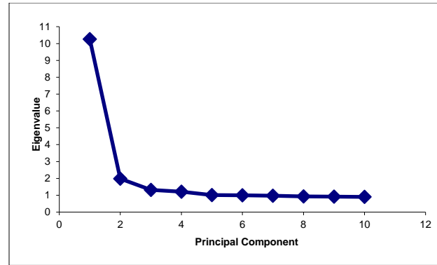
P-2. English Grade 10 Principal Components Scree Plot
