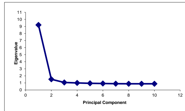
P-8. Science Grade 10 Principal Components Scree Plot
