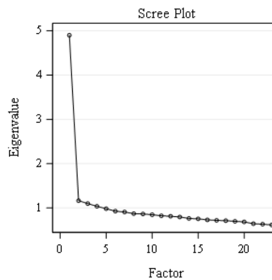
Figure K.8. Science Grade 10 Principal Components Scree Plot
